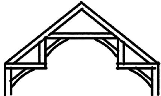
HAMMERBEAM TRUSS
