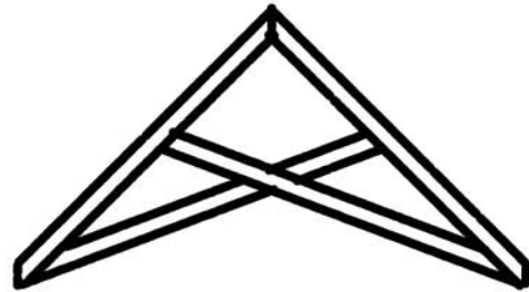
SCISSOR TRUSS
